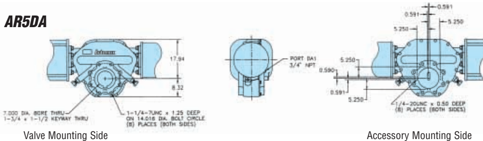
Valve Mounting Side
