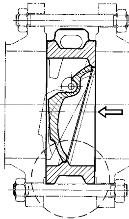
Fig. 3 Incorrect Installation
