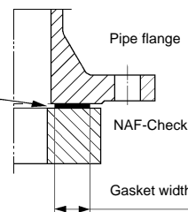
Fig. 4 Recommended gasket widths
