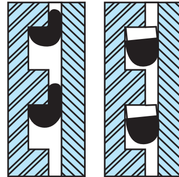
Without back-up rings
