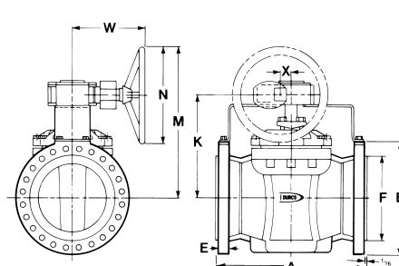
8 in (200 mm) thru 18 in (450 mm) G431H – Class 300
