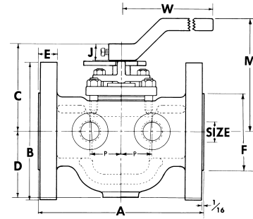
Stem Configuration 1/2 in (15 mm) to 6 in (150 mm) flats
