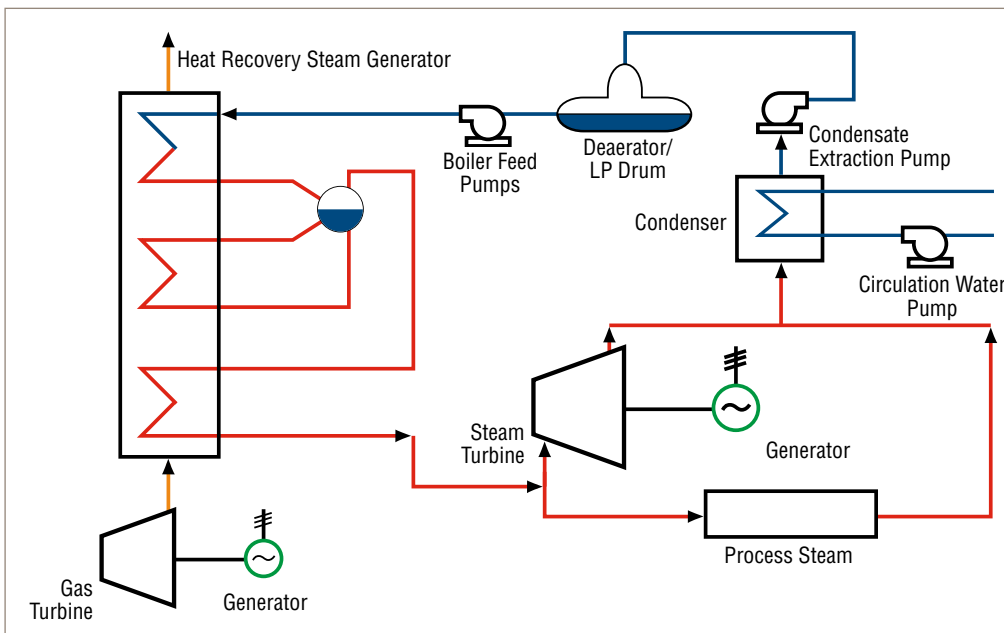
Figure 1 – Simplified Combined Cycle Power Plant
