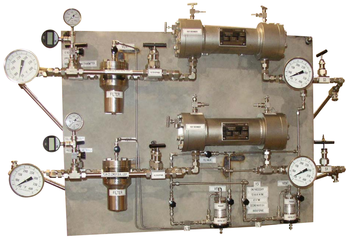
Dual Plan 23 Seal Cooling and Monitoring Panel
