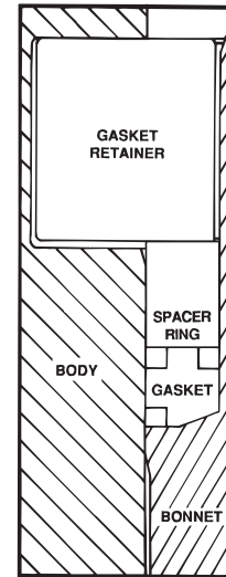
Composite Pressure-Seal Construction
