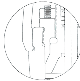
Pressure Seal Detail
