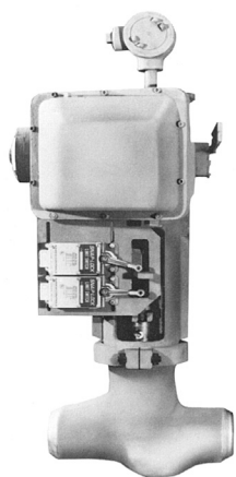
4" 600# Globe Valve
