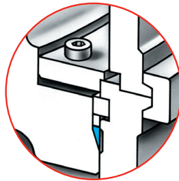
Pressure Seal Design
