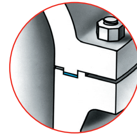
Bolted Bonnet Design
