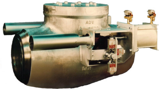
Tilting-Disc Check
