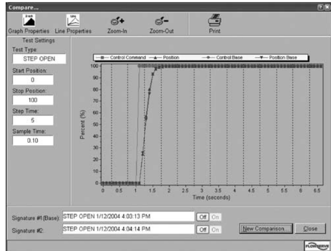
Figure 11: Performance Test
