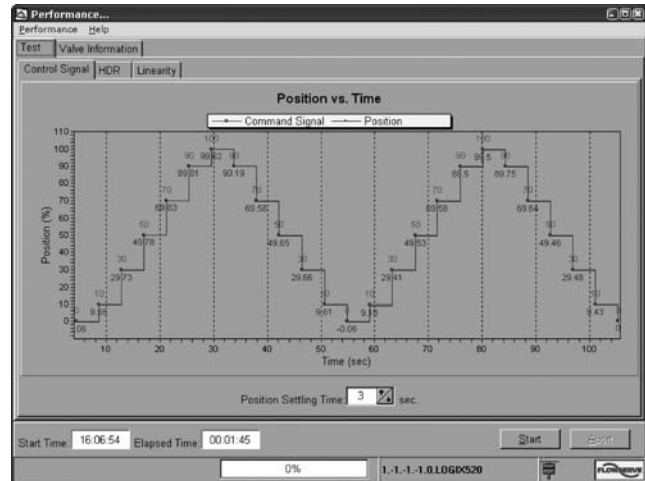
Figure 11: Performance Test
