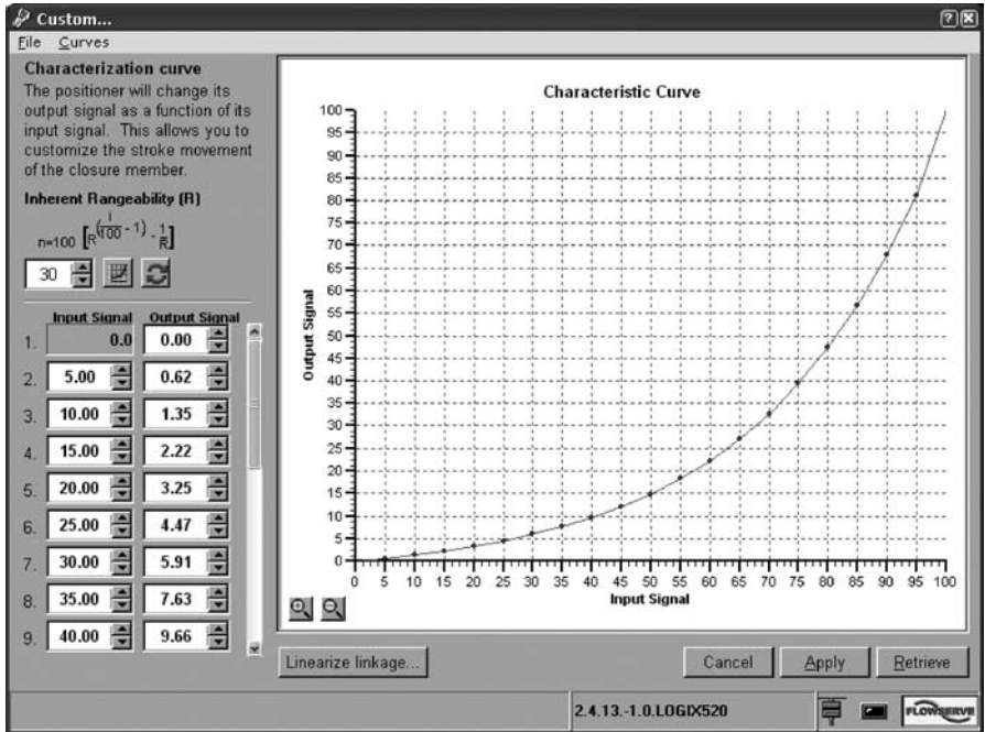
Figure 7: 21-point Characterization Curve
