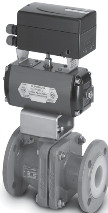
Figure 17: Logix 500si Series Positioner Acc. Industry-standard VDI/VDE 3845 (DIN ISO 5211) Mounting.
