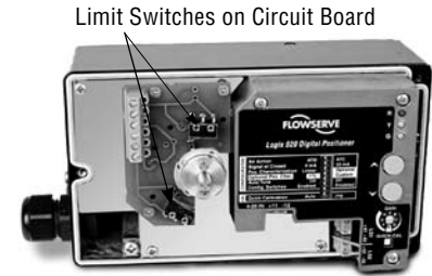
Figure 12: Optional Internal Limit Switches
