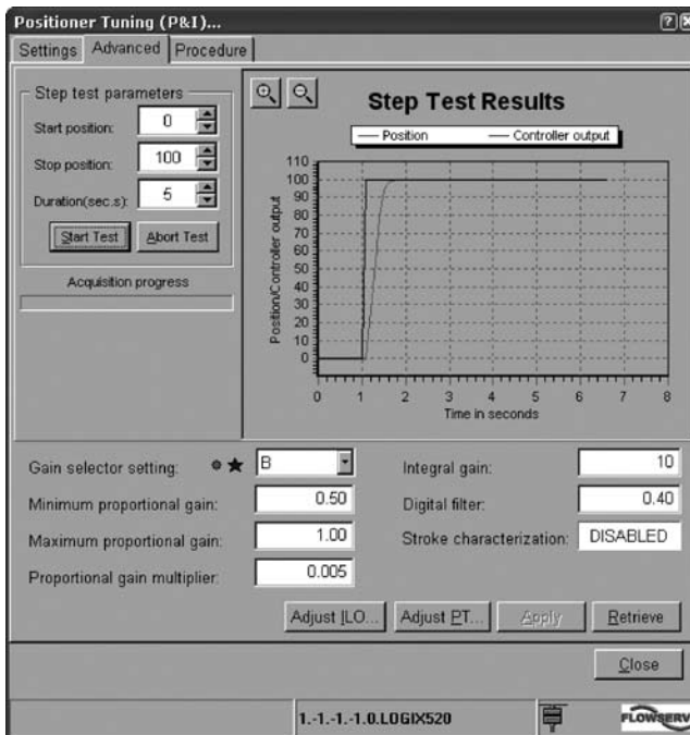
Figure 8: Manual Tuning with User Interface
