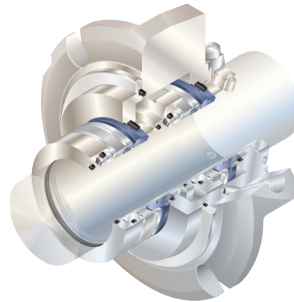
ISC2-BX Single cartridge metal bellows seal for crystallizing fluid conditions
