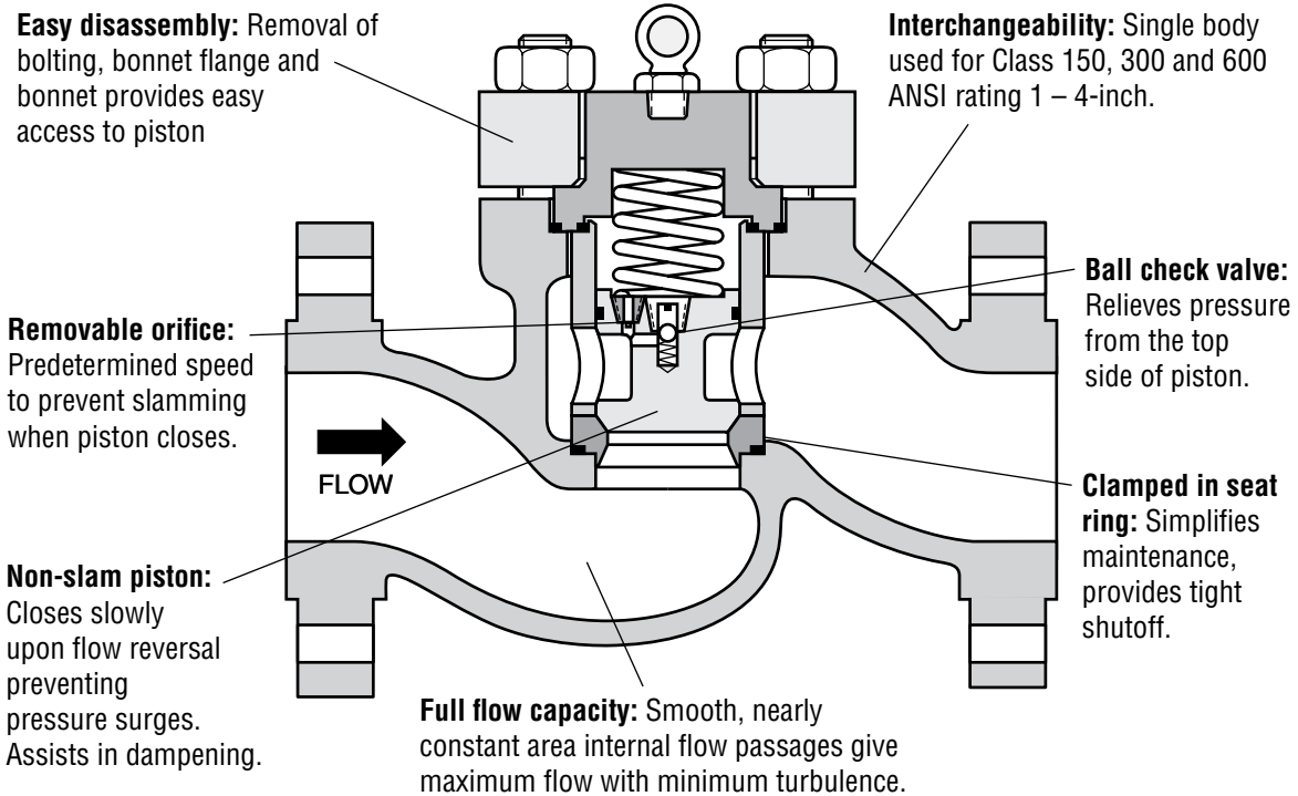
Figure 1: Non-Slam Piston Type Features
