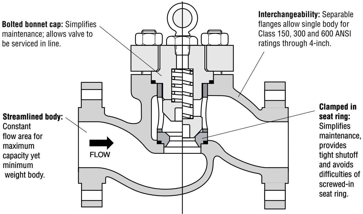
Figure 2: Plug Type Features
