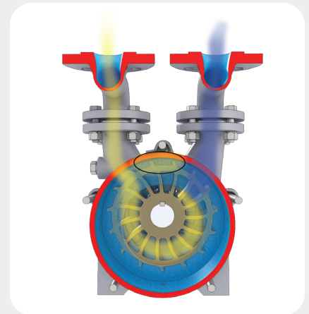
The process material leaves the compressor while the separated waste gas is recovered for additional processing or utilized as fuel.
