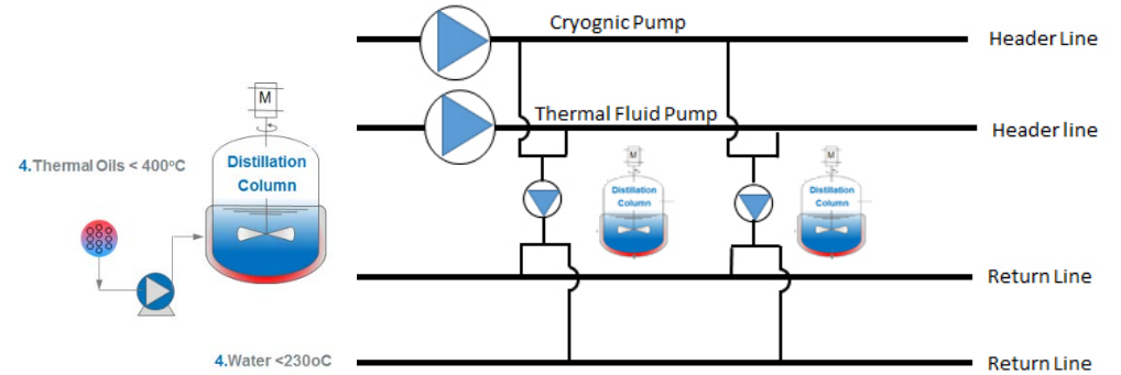
3. Thermal Heating Pumps
