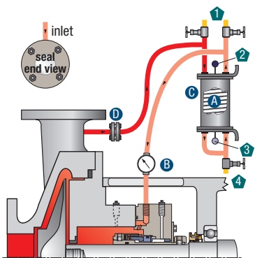
A - cooling coils B - temperature indicator C - cooler D - orifice 1 - vents, normally closed 2 - cooling out 3 - cooling in 4 - drain, normally closed
