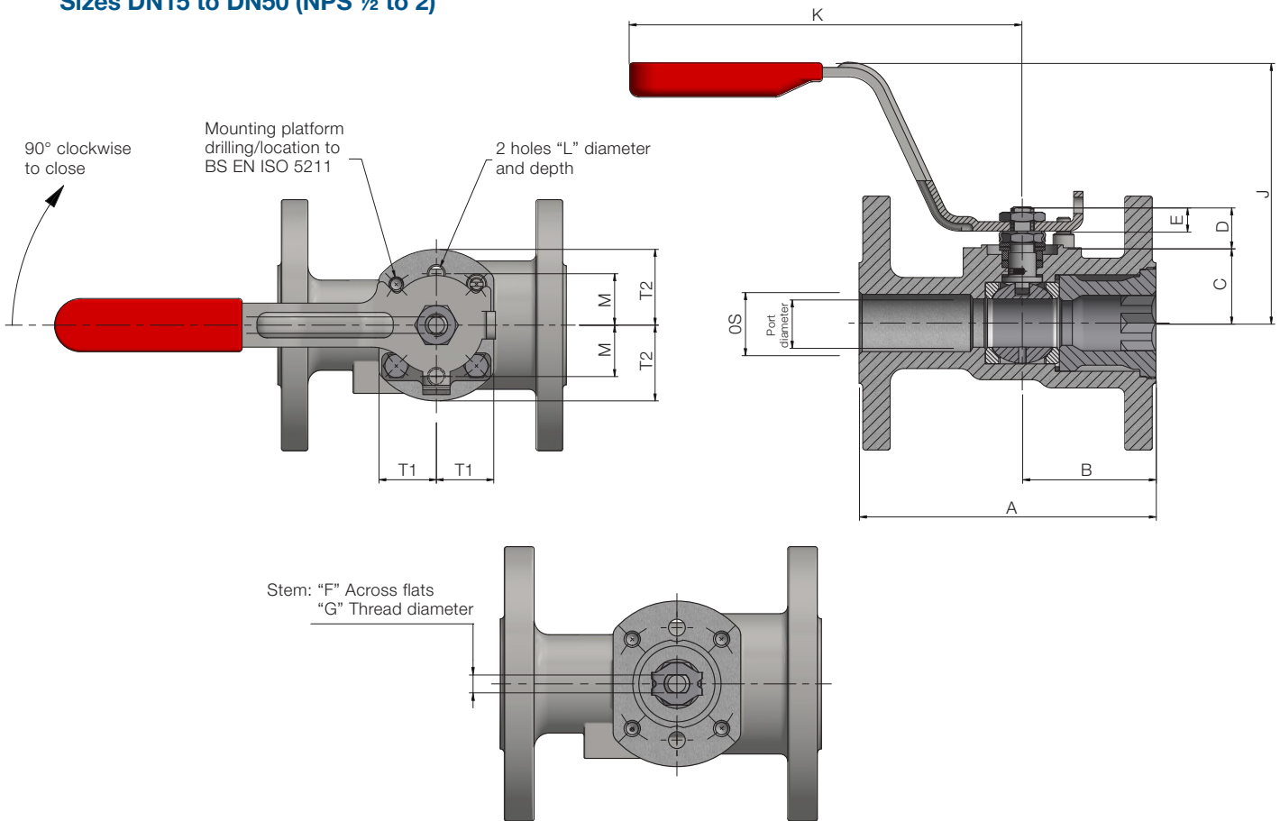
Dimensions indicated in mm (in.)
