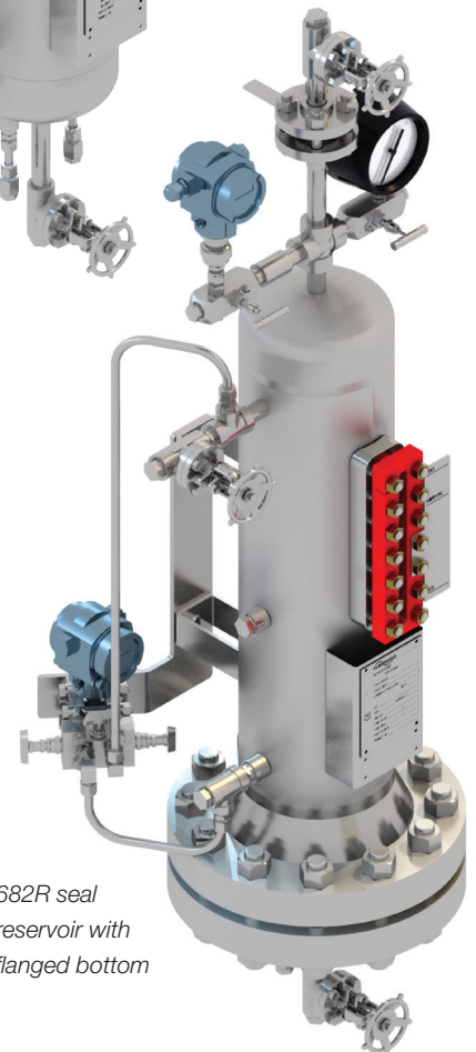
682R seal reservoir with elliptical bottom
