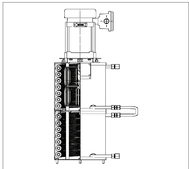
Figure 2. A625 Seal Cooler operating principle
