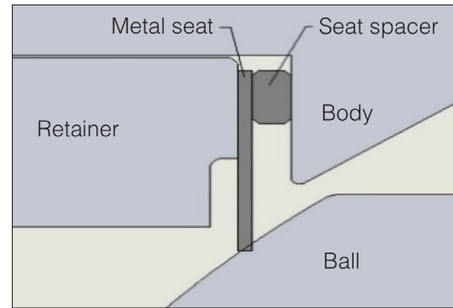
Figure 1: Metal seat
