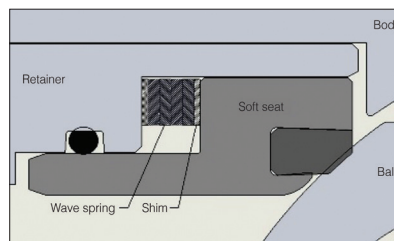
Figure 4: Heavy-duty soft seat
