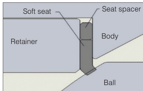
Figure 2: Soft seat
