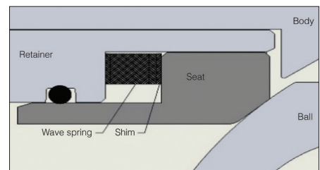
Figure 5: Heavy-duty metal seat
