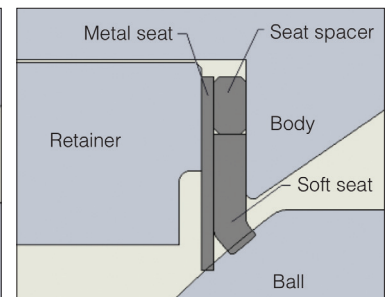
Figure 3: Dual seat
